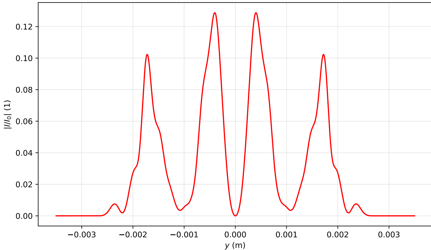
Intensity profile I(x=0, y, z=2.468)/I_0 , P_{in}=9.0P_{cr} , artificial time
